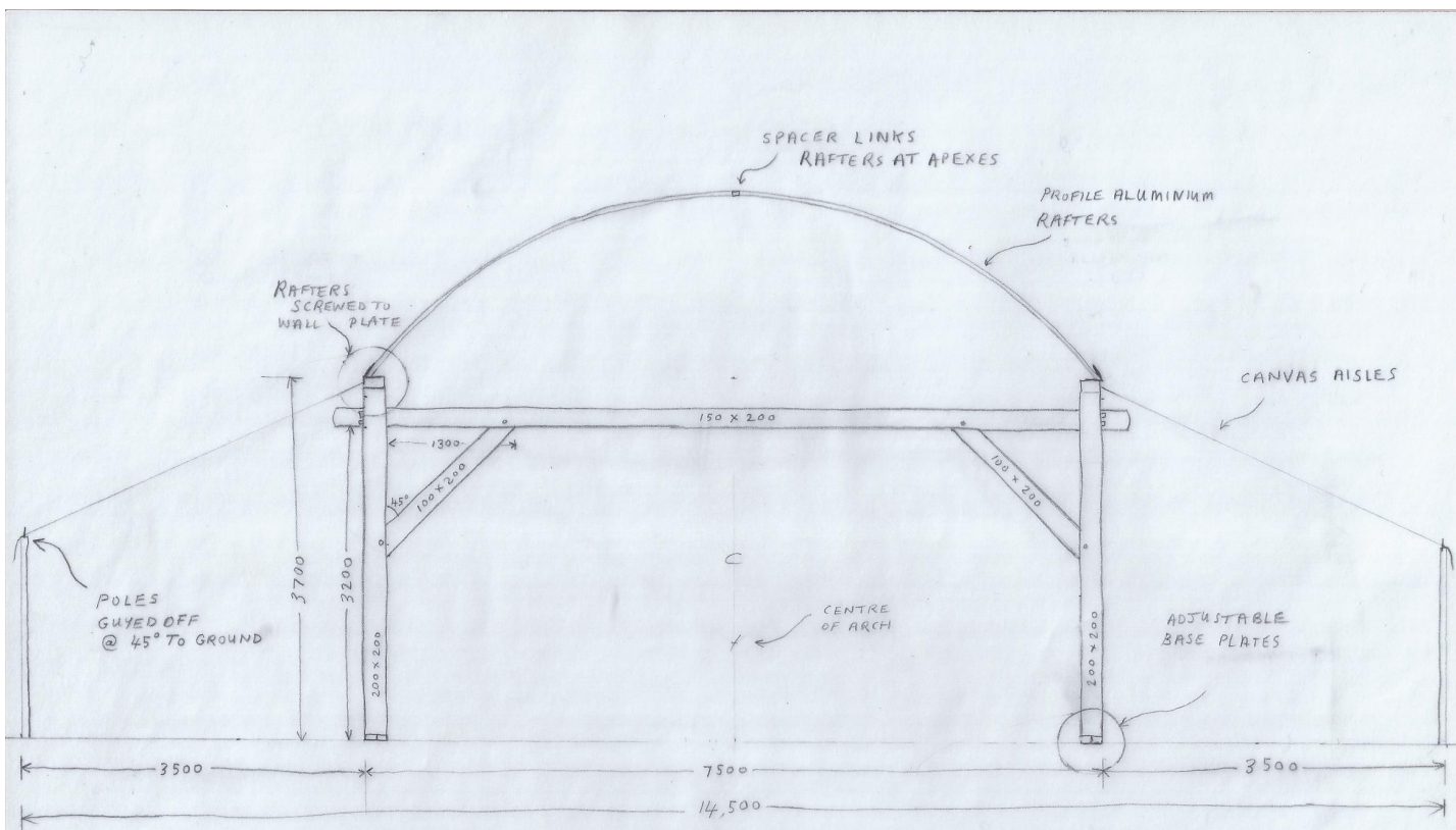
TRAVELLING BARN SCALE 1:50 DOUGLAS FIR DRAWING NO 1 © GABRIEL LANGLANDS 2011
